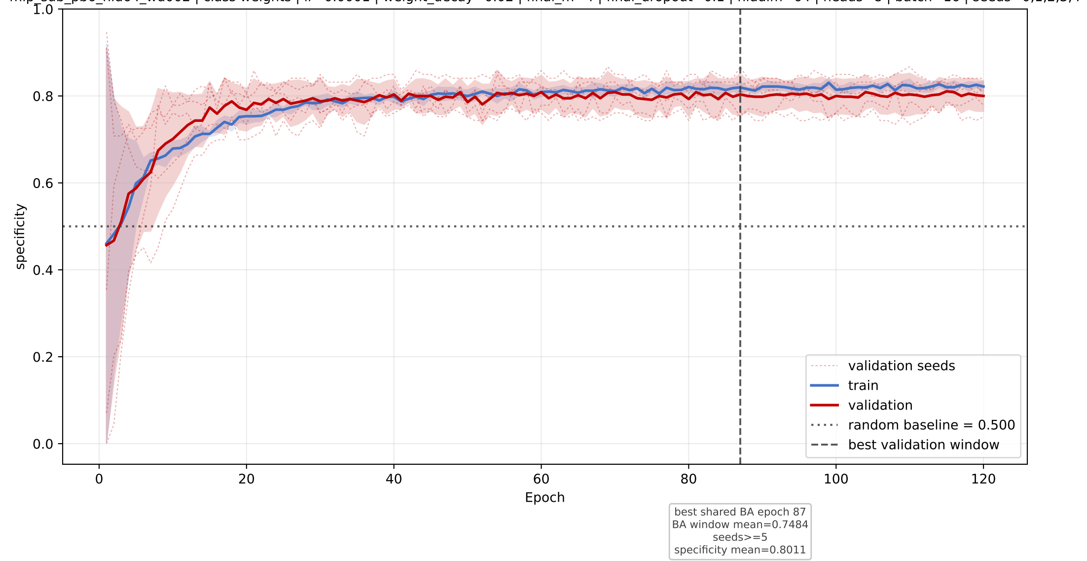
PG: mean specificity learning curve across seeds
