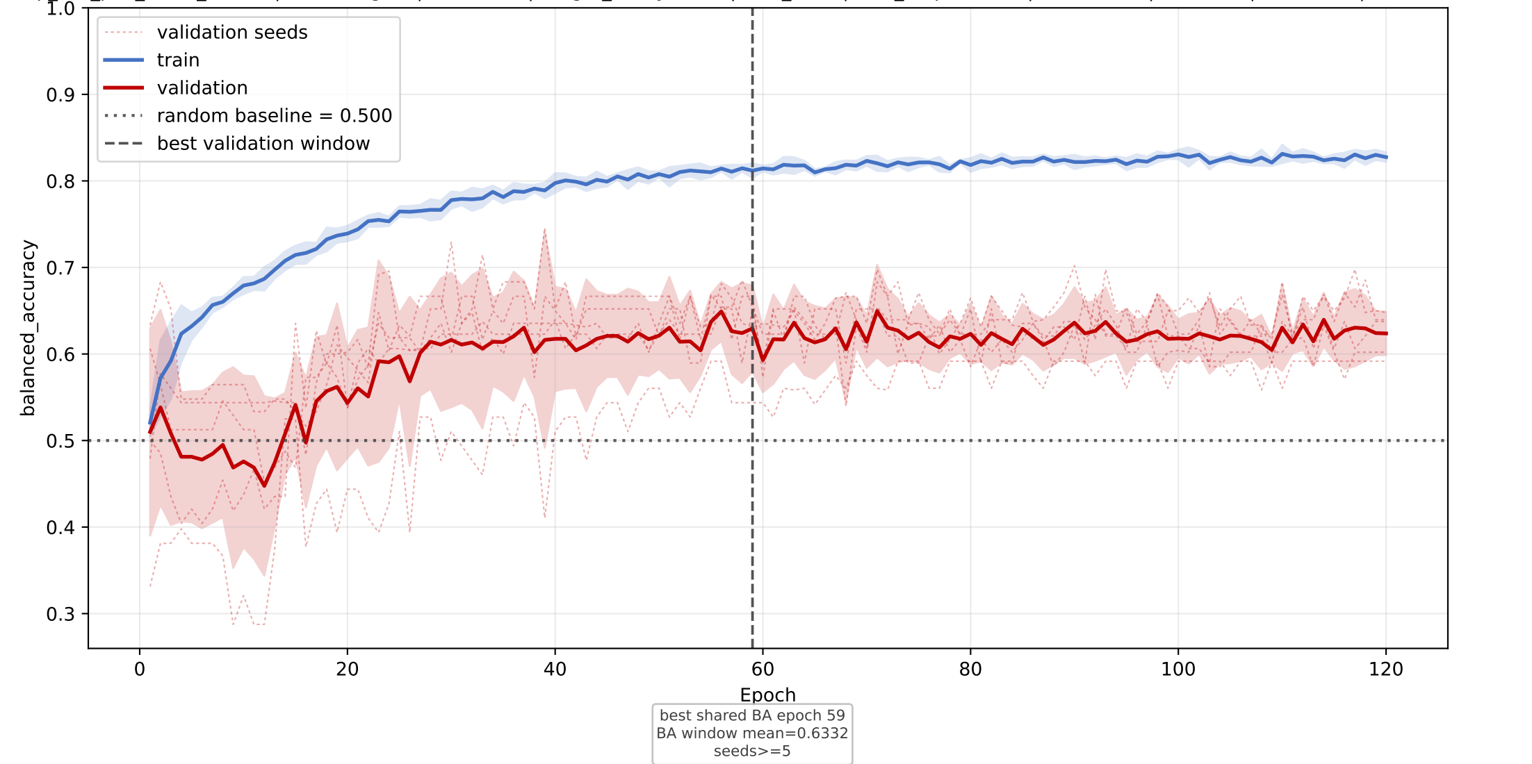
LPC+LPE+LPG: mean balanced_accuracy learning curve across seeds
