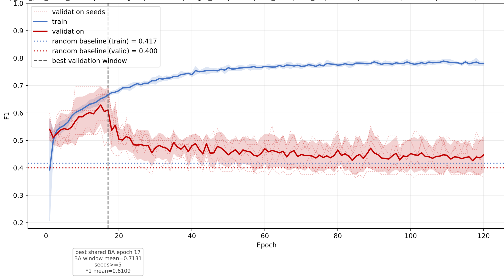
PA: mean F1 learning curve across seeds
