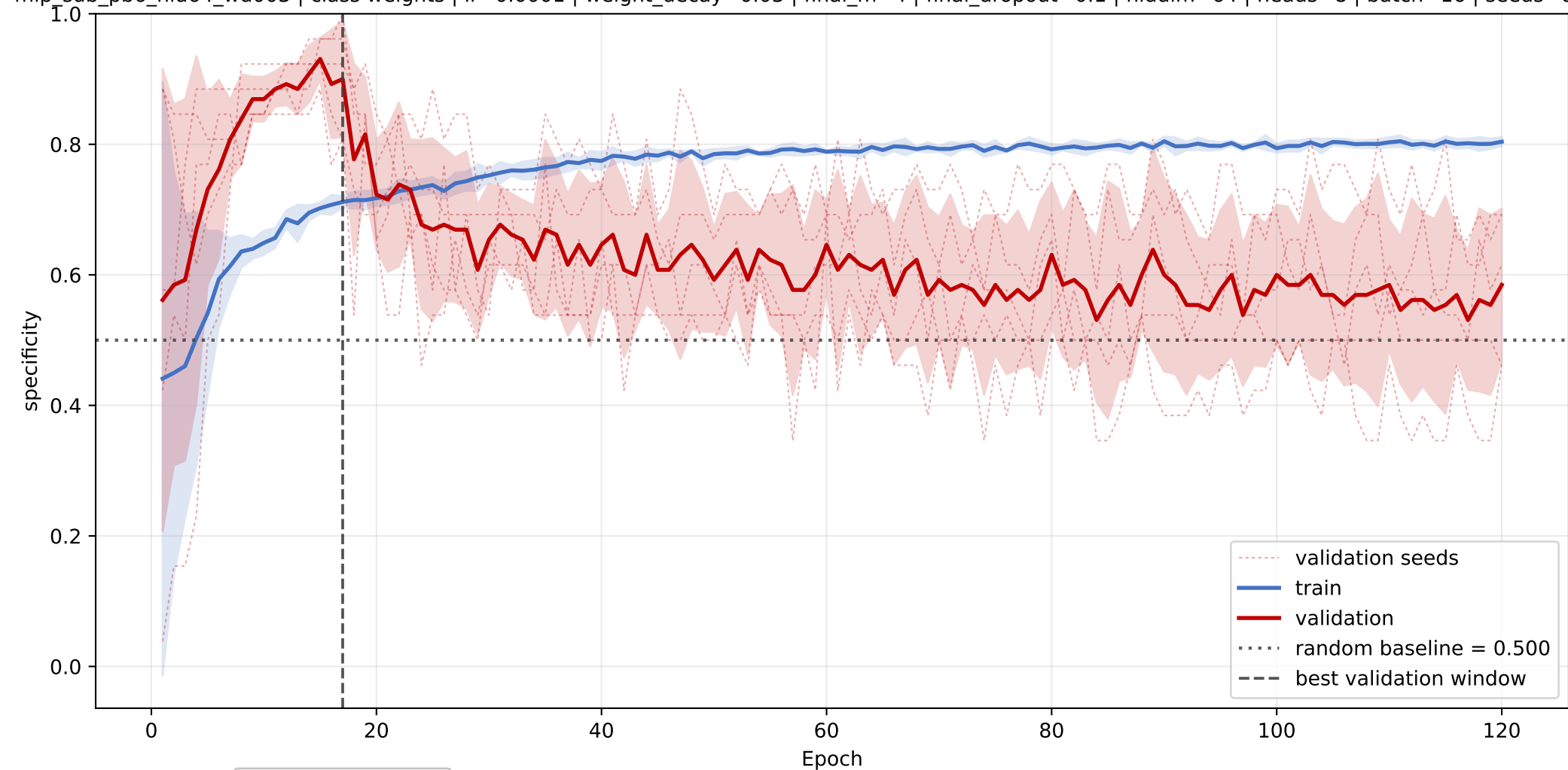
PA: mean specificity learning curve across seeds
