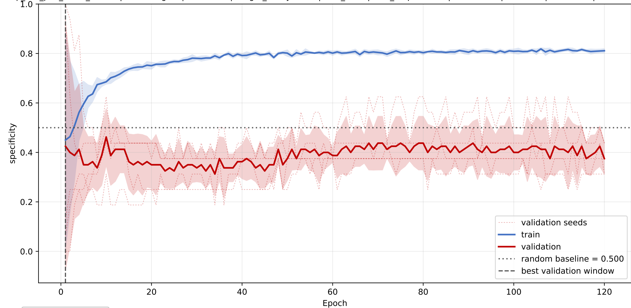
PS+PGP+DAG+TAG: mean specificity learning curve across seeds
