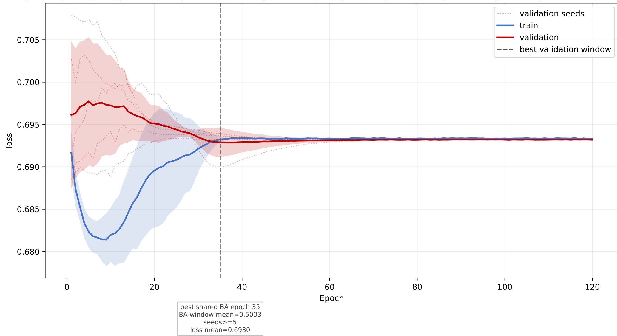
FA: mean loss learning curve across seeds
