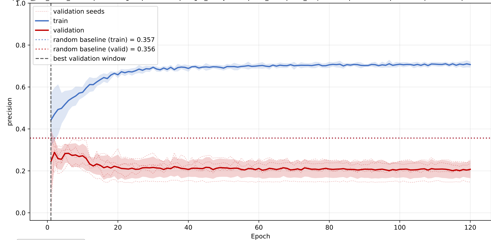
PC: mean precision learning curve across seeds
