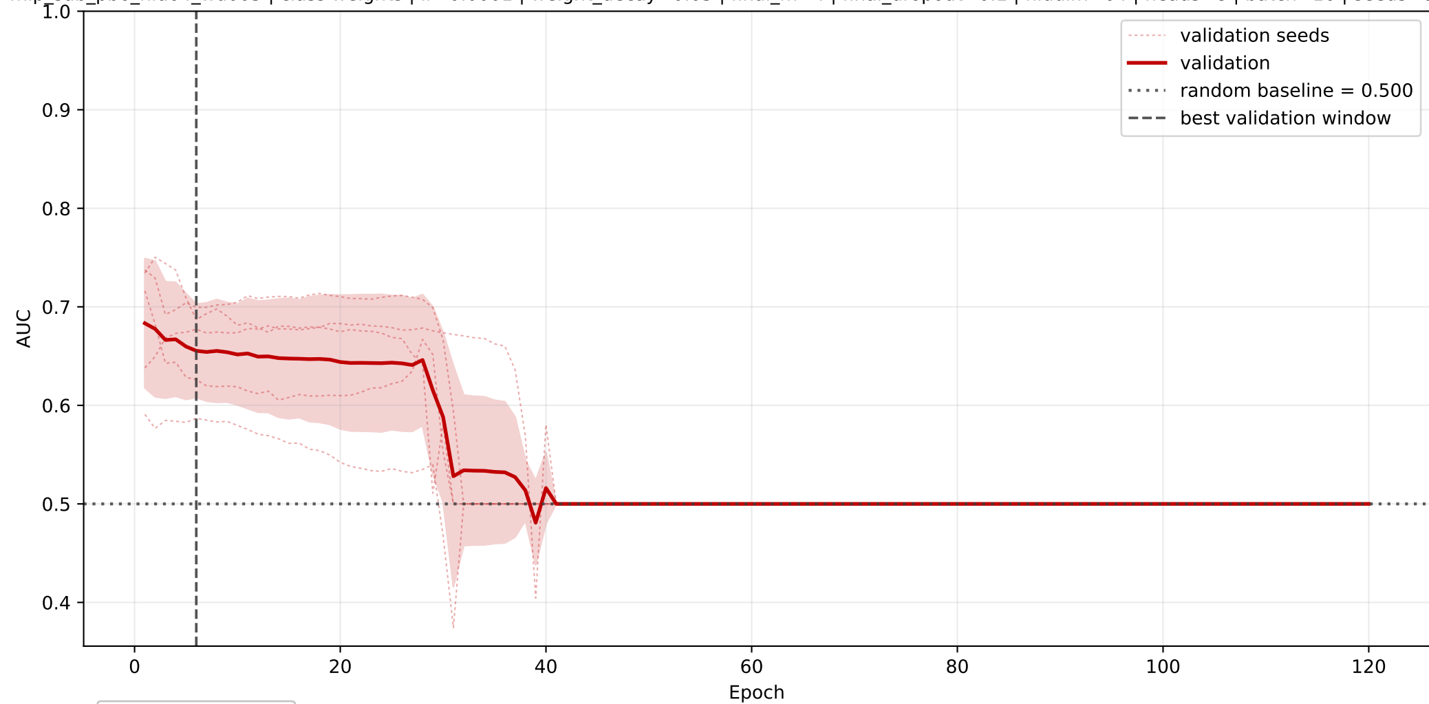
PG: mean AUC learning curve across seeds
