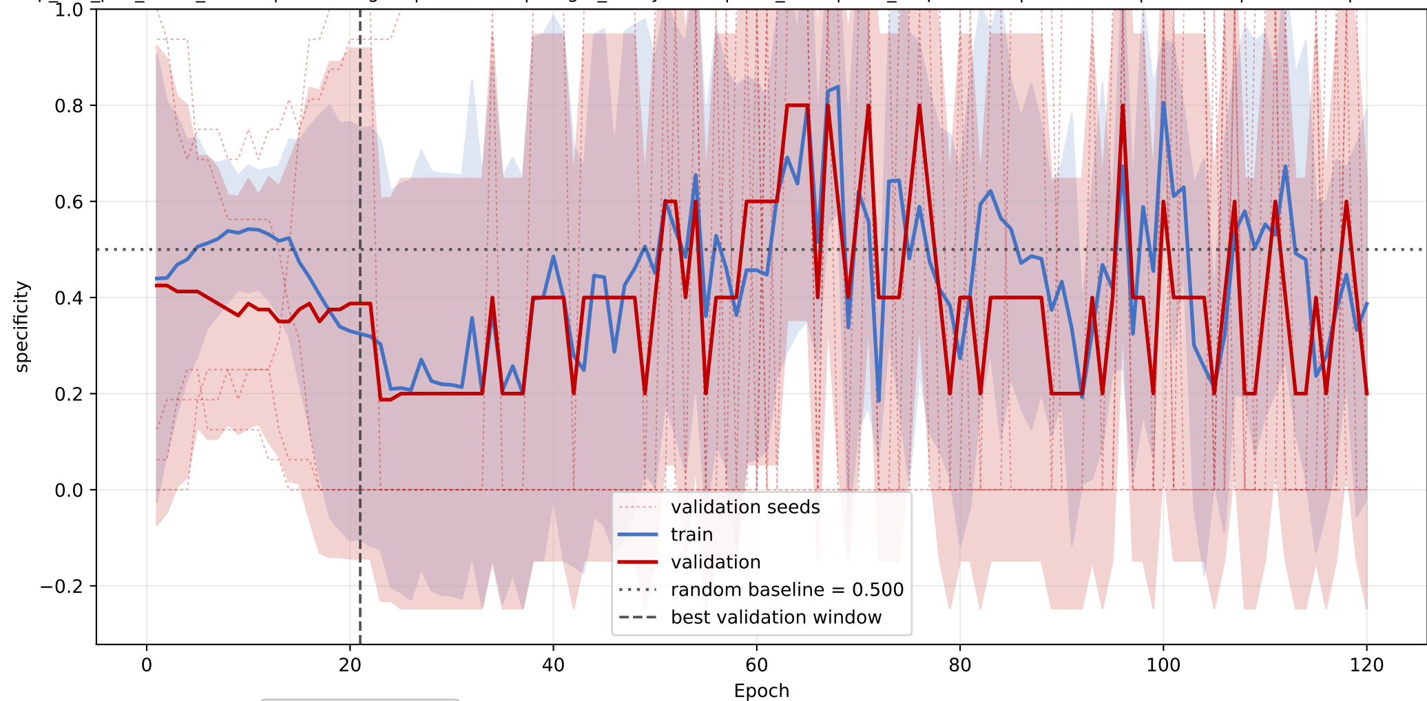
PS+PGP+DAG+TAG: mean specificity learning curve across seeds
