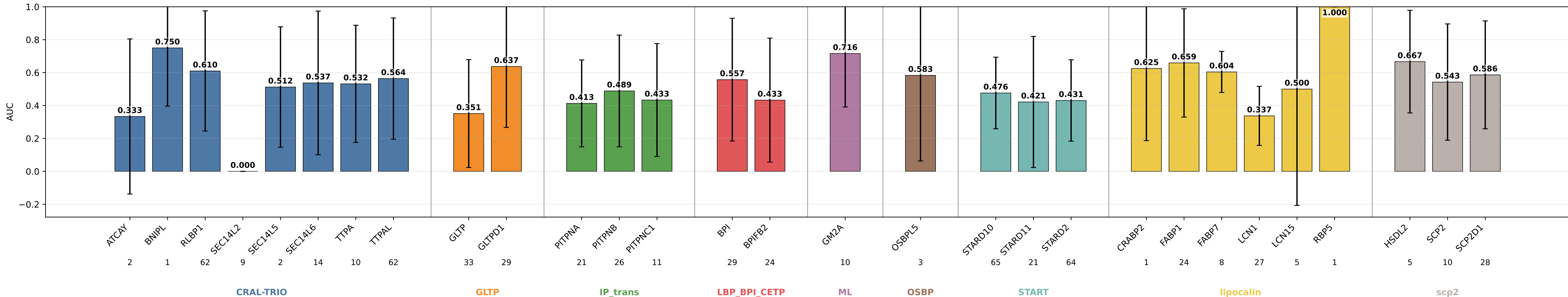
mlp_sub_pb6_hid64_wd005 AUC by subgroup mlp_sub_pb6_hid64_wd005 | class weights | lr=0.0001 | weight_decay=0.05 | final_m=4 | final_dropout=0.1 | hiddim=64 | heads=8 | batch=16 | ep=120 | seeds=0,1,2,3,4
