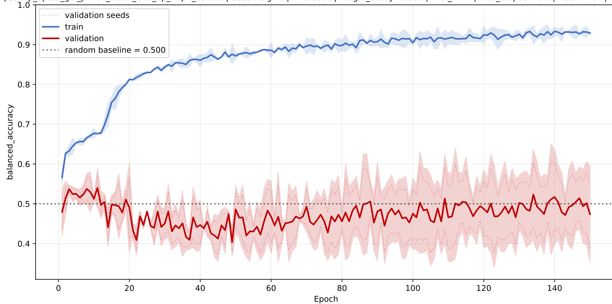
START: mean balanced_accuracy learning curve across seeds
