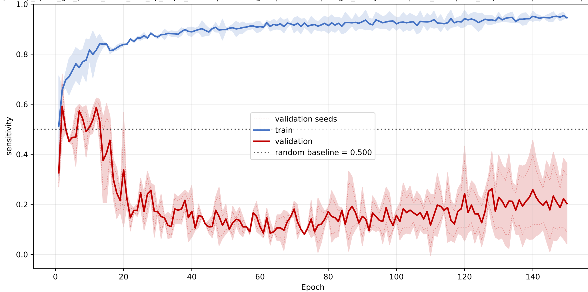
START: mean sensitivity learning curve across seeds
