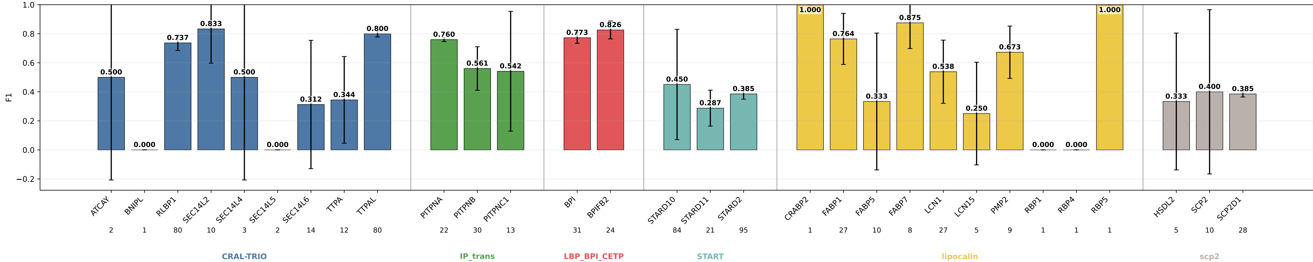
bbp_fa_edge_curent_nps3mlp_dpt01_gm_plm64_hid64_GRL_dp_rmpft_batch8 F1 by subgroup bbp_fa_edge_curent_nps3mlp_dpt01_gm_plm64_hid64_GRL_dp_rmpft_batch8 | class weights | lr=0.0001 | weight_decay=0.001 | final_m=4 | final_dropout=0.1 | hiddim=64 | heads=8 | batch=8 | ep=150 | seeds=0,1
