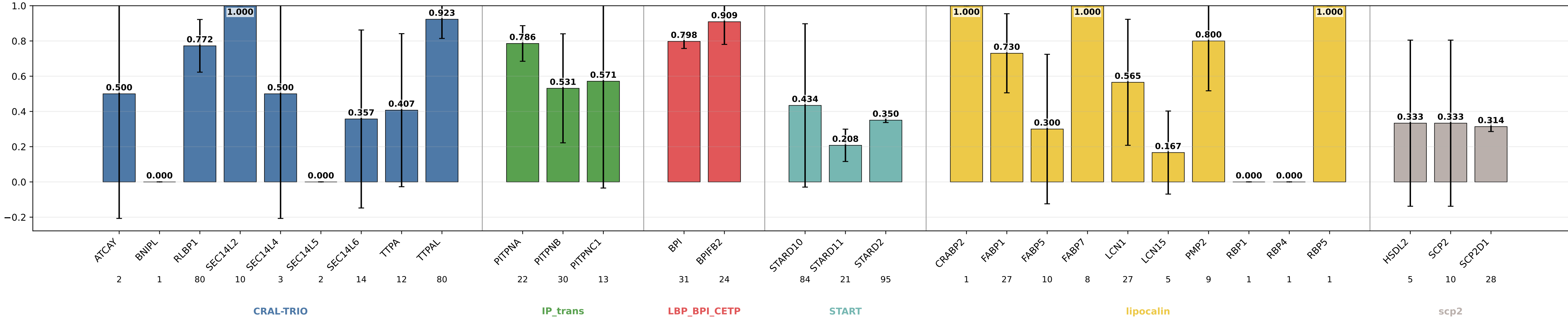
bbp_fa_edge_curent_nps3mlp_dpt01_gm_plm64_hid64_GRL_dp_rmpft_batch8 sensitivity by subgroup bbp_fa_edge_curent_nps3mlp_dpt01_gm_plm64_hid64_GRL_dp_rmpft_batch8 | class weights | lr=0.0001 | weight_decay=0.001 | final_m=4 | final_dropout=0.1 | hiddim=64 | heads=8 | batch=8 | ep=150 | seeds=0,1
