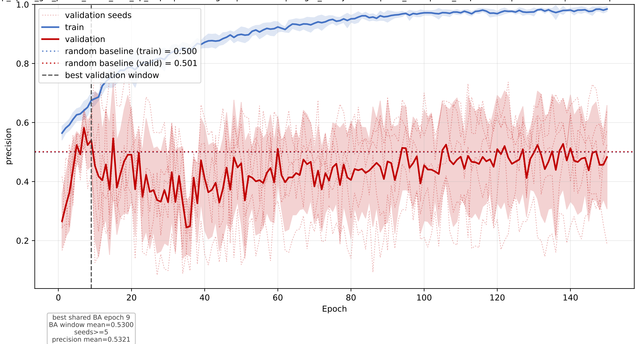
CRAL-TRIO: mean precision learning curve across seeds
