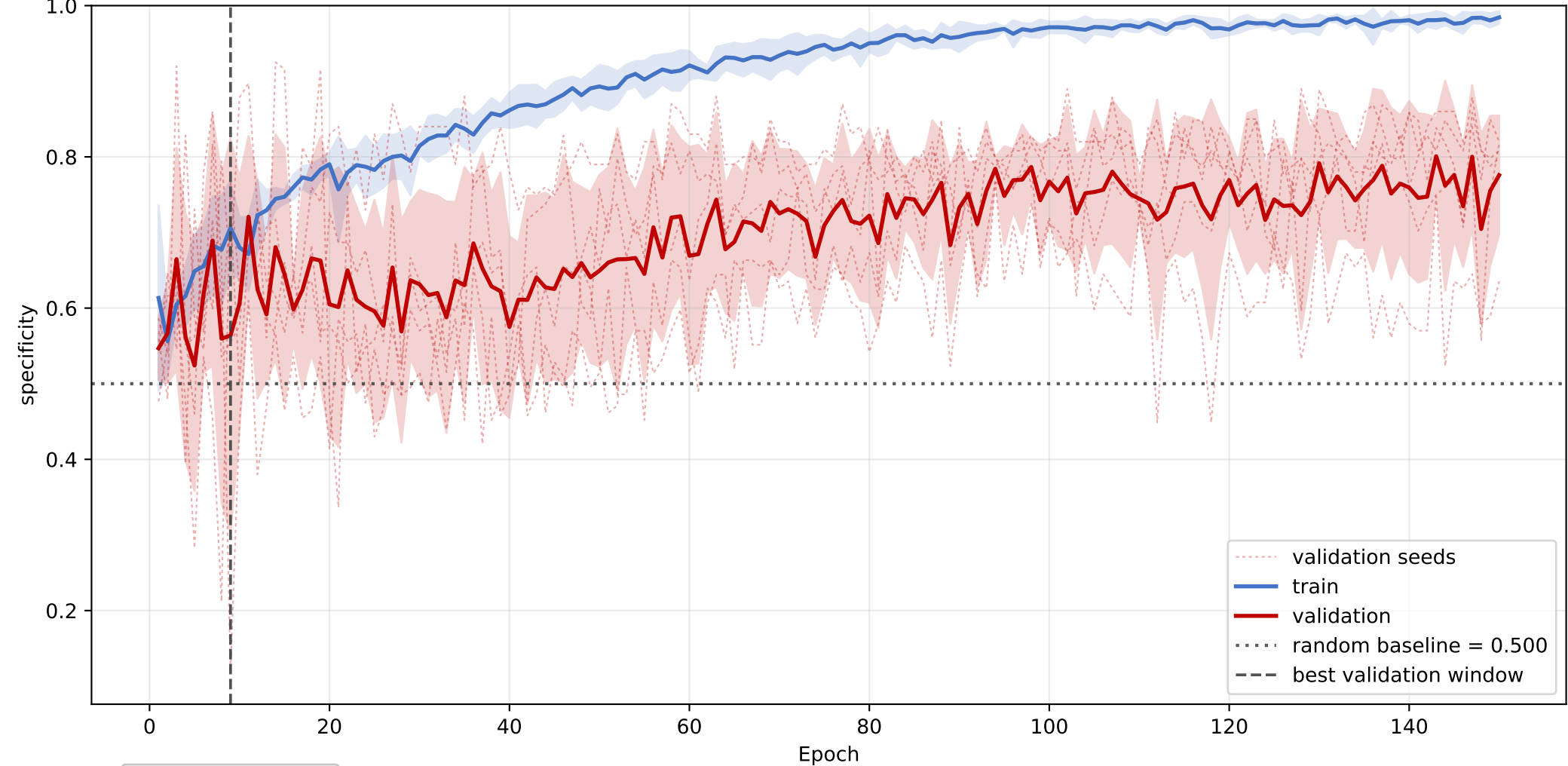
CRAL-TRIO: mean specificity learning curve across seeds
