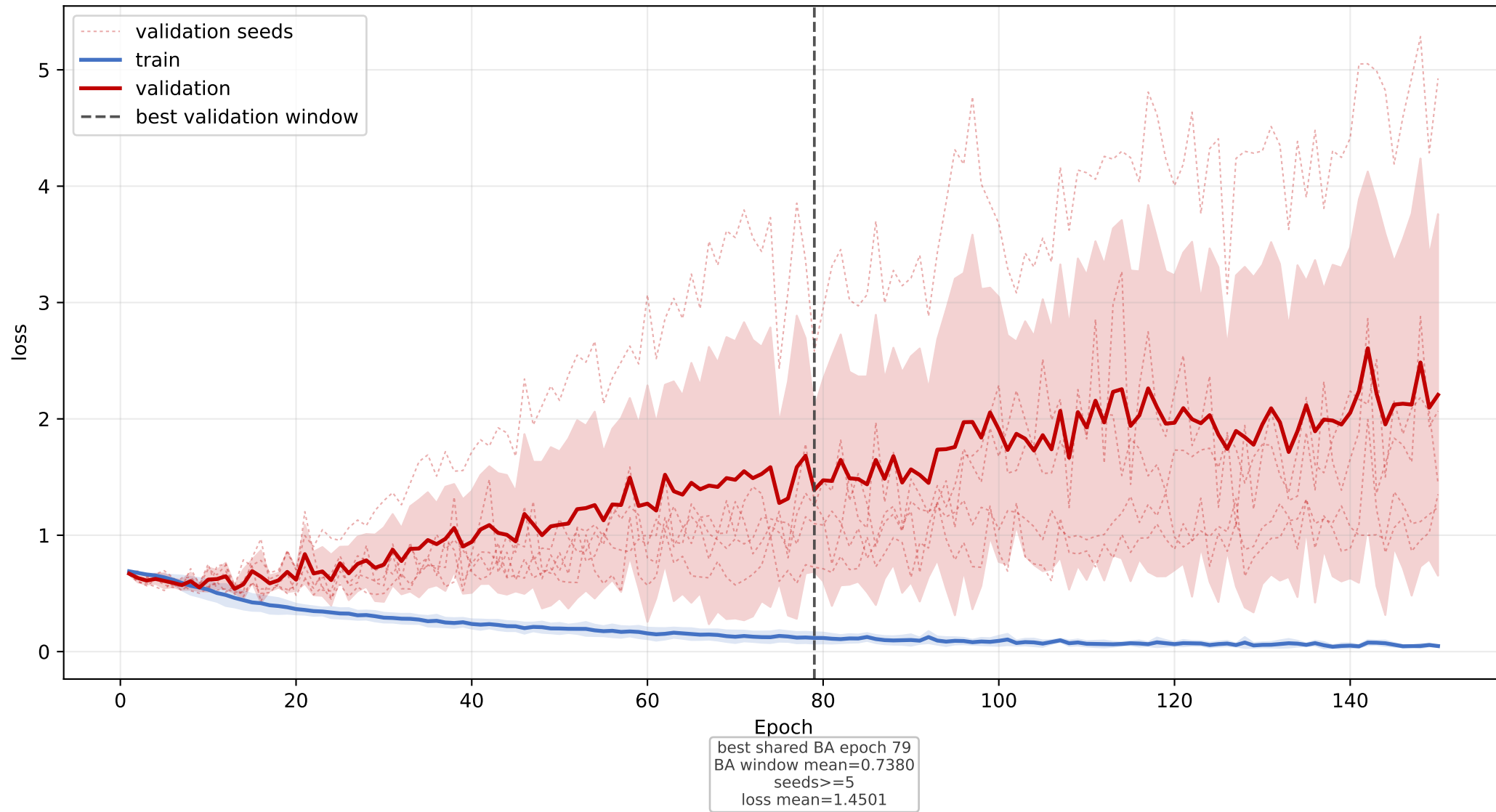
LBP_BPI_CETP: mean loss learning curve across seeds
