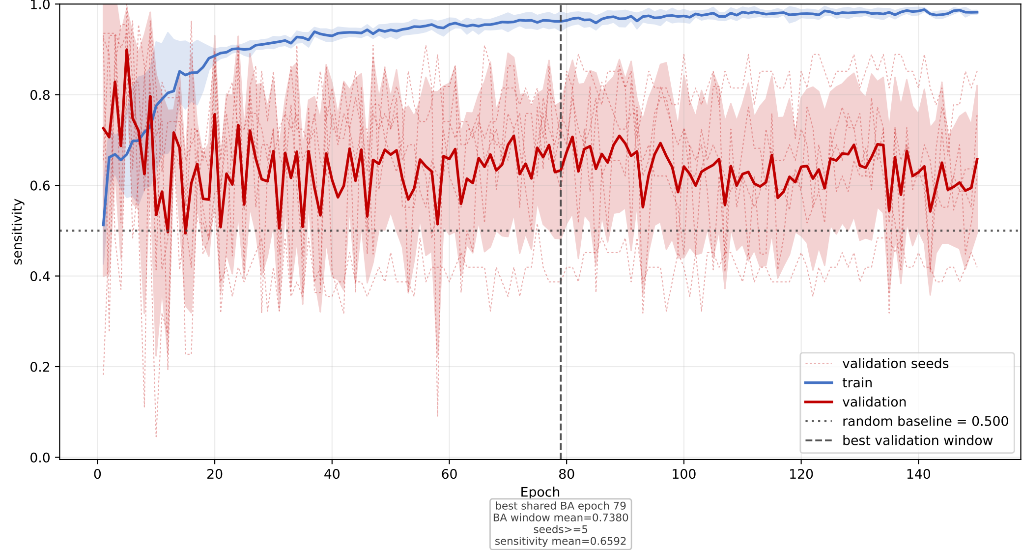
LBP_BPI_CETP: mean sensitivity learning curve across seeds
