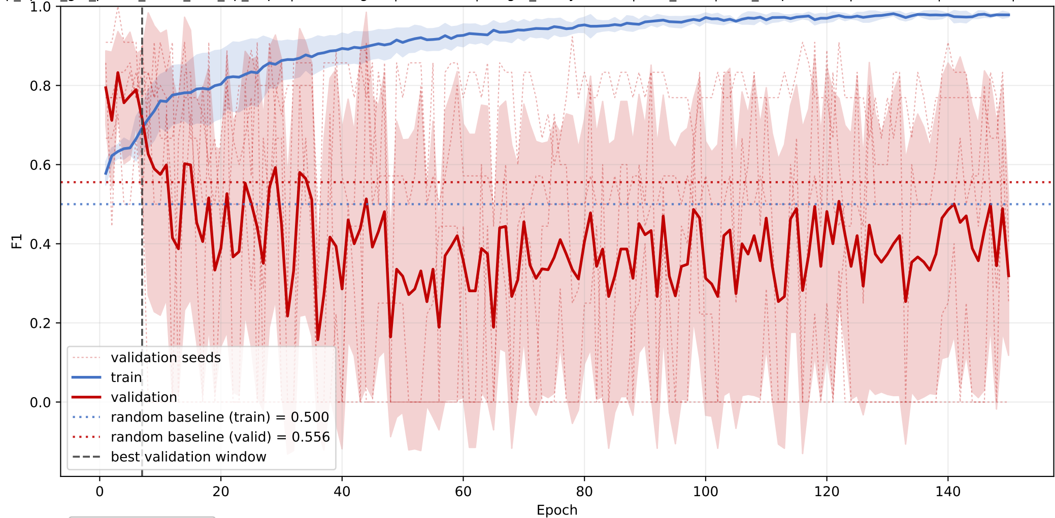
OSBP: mean F1 learning curve across seeds
