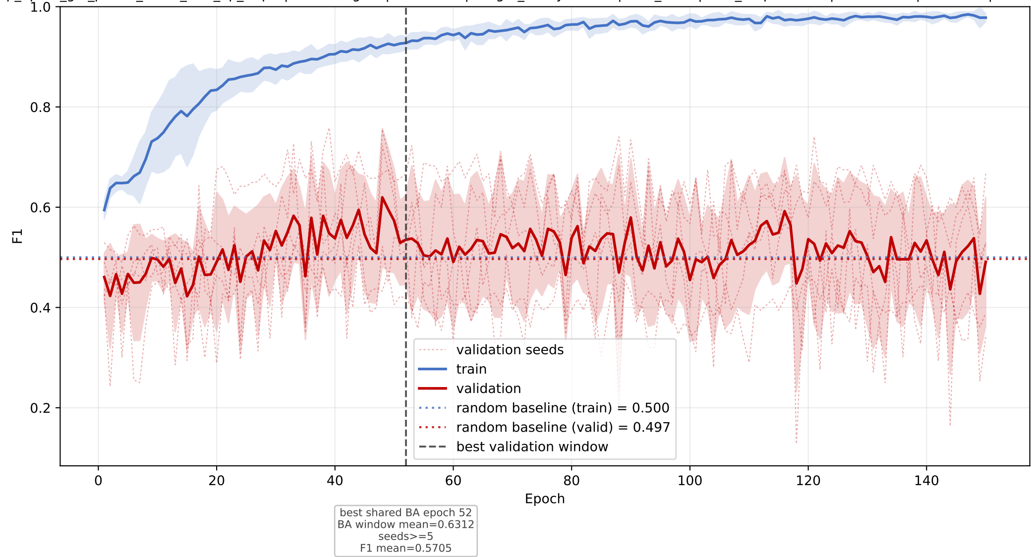
lipocalin: mean F1 learning curve across seeds
