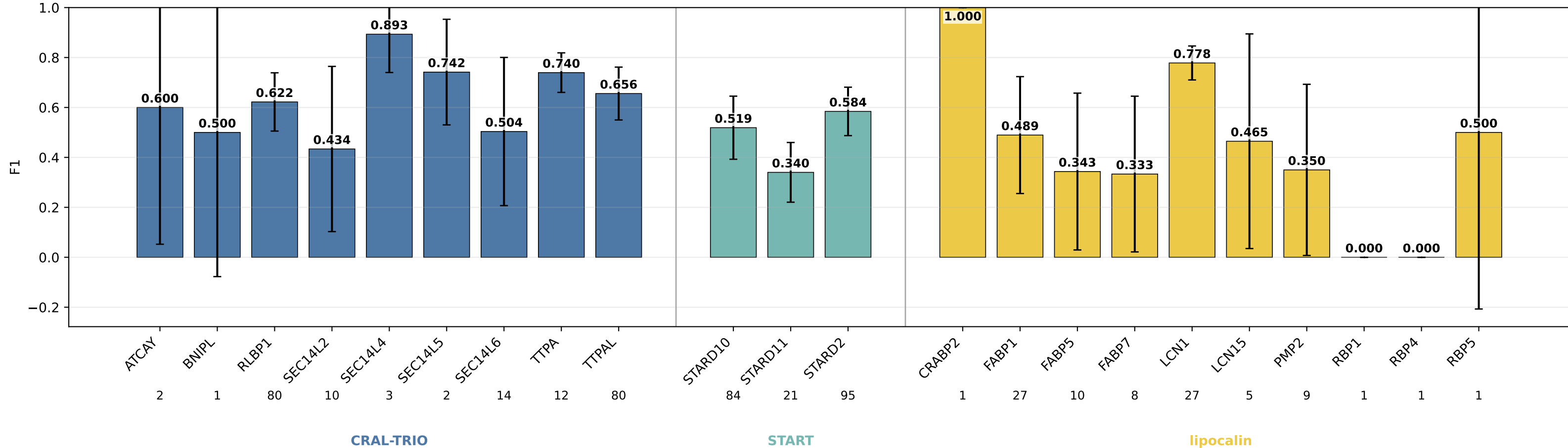
bbp_fa_nps3mlp_dpt01_wd0001_gm_plm64_hid64_GRL_dp_rmpft_lambda2 F1 by subgroup
