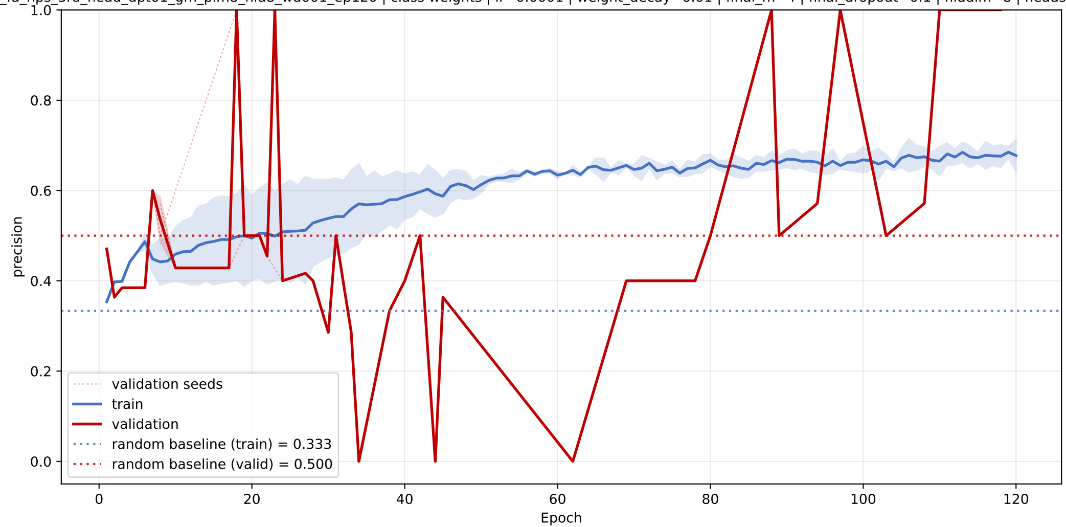
GLTP: mean precision learning curve across seeds
