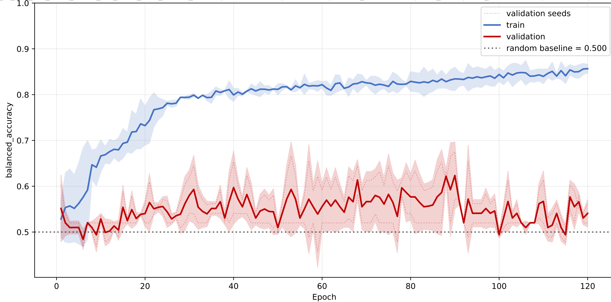
LBP_BPI_CETP: mean balanced accuracy learning curve across seeds
