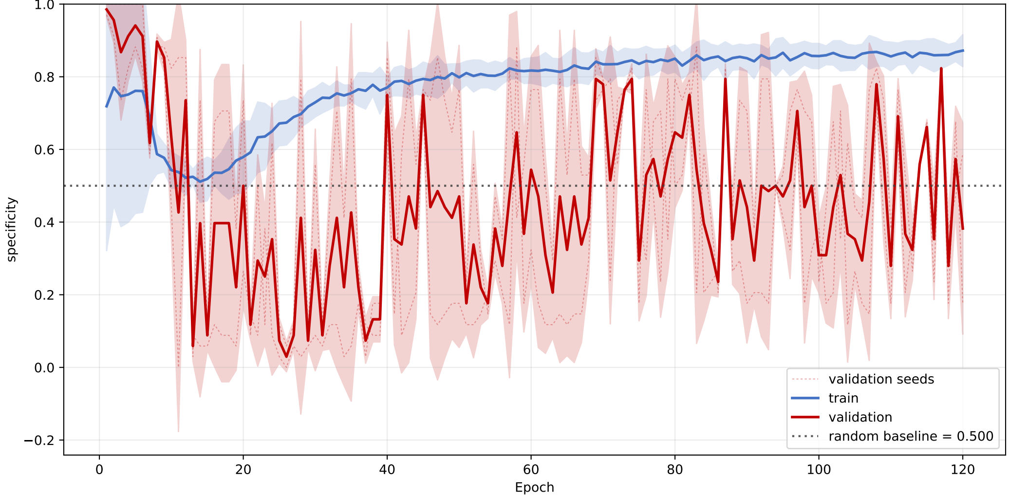
scp2: mean specificity learning curve across seeds
