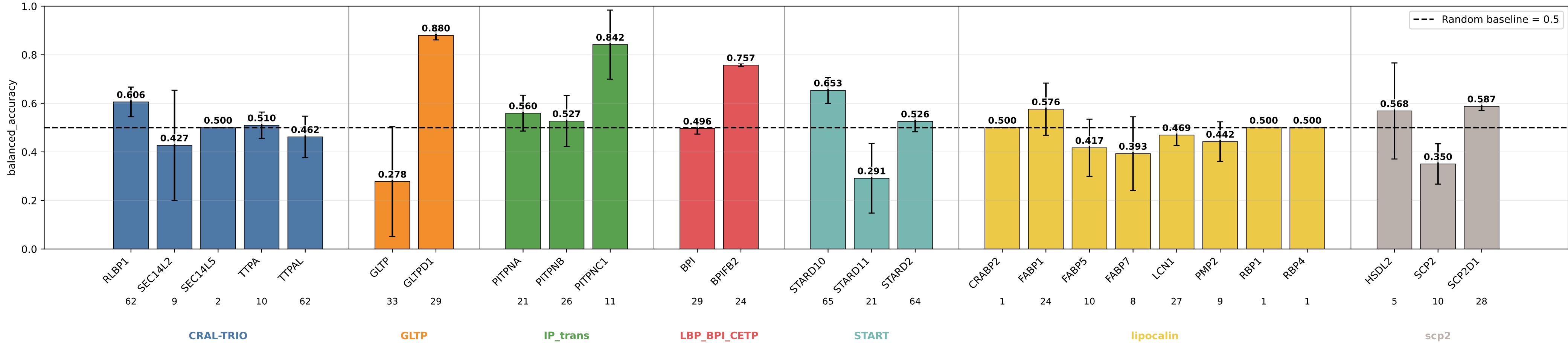
bbp_dcs_rand_smd_fa_nps_bilinear_fusion_dpt01_gm_plm8_hid8_wd001_ep120 balanced_accuracy by subgroup bbp_dcs_rand_smd_fa_nps_bilinear_fusion_dpt01_gm_plm8_hid8_wd001_ep120 | class weights | lr=0.0001 | weight_decay=0.01 | final_m=4 | final_dropout=0.1 | hiddim=8 | heads=8 | batch=16 | ep=120 | seeds=0,1,2,3
