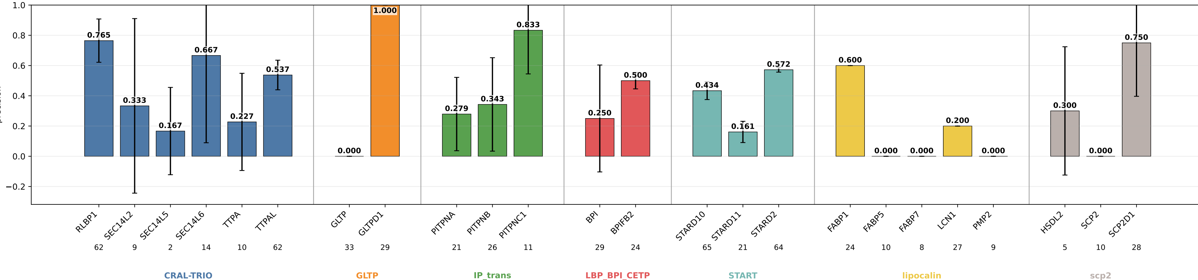
bbp_dcs_rand_smd_fa_nps_bilinear_fusion_dpt01_gm_plm8_hid8_wd001_ep120 precision by subgroup bbp_dcs_rand_smd_fa_nps_bilinear_fusion_dpt01_gm_plm8_hid8_wd001_ep120 | class weights | lr=0.0001 | weight_decay=0.01 | final_m=4 | final_dropout=0.1 | hiddim=8 | heads=8 | batch=16 | ep=120 | seeds=0,1,2,3
