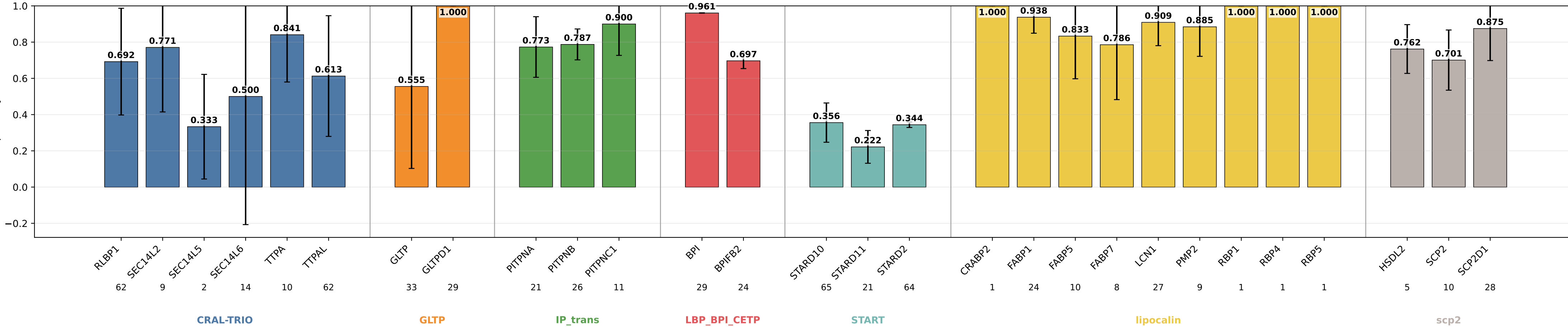
bbp_dcs_rand_smd_fa_nps_bilinear_fusion_dpt01_gm_plm8_hid8_wd001_ep120 specificity by subgroup bbp_dcs_rand_smd_fa_nps_bilinear_fusion_dpt01_gm_plm8_hid8_wd001_ep120 | class weights | lr=0.0001 | weight_decay=0.01 | final_m=4 | final_dropout=0.1 | hiddim=8 | heads=8 | batch=16 | ep=120 | seeds=0,1,2,3
