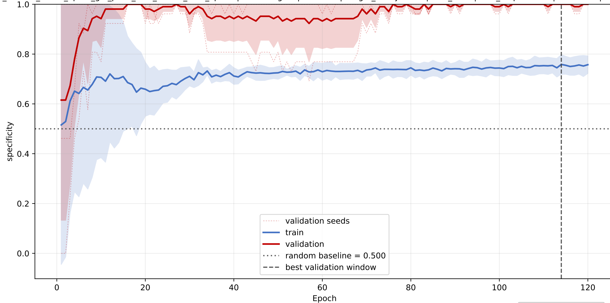
GLTP: mean specificity learning curve across seeds
