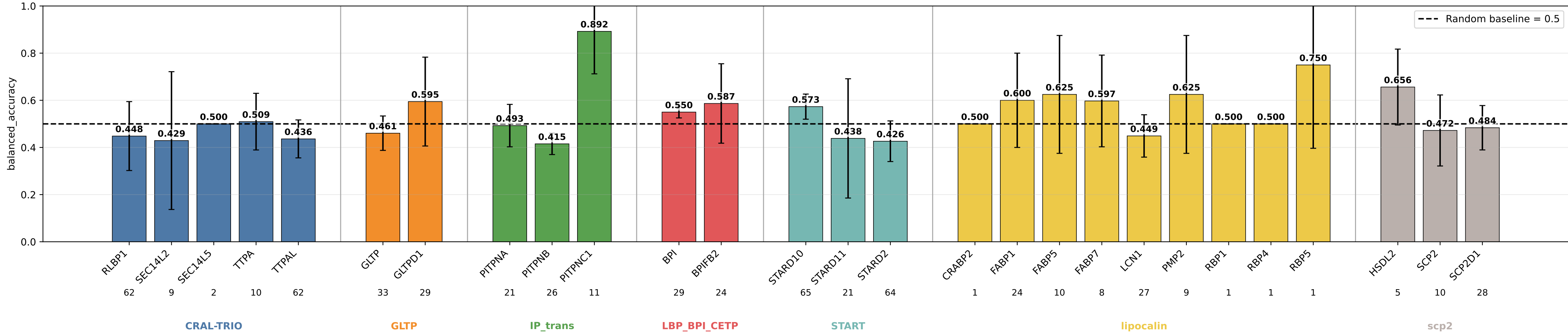
bbp_dcs_rand_smd_fa_nps_bilinear_fusion_dpt01_gm_plm8_hid8_wd001_lre-5_ep120 balanced_accuracy by subgroup bbp_dcs_rand_smd_fa_nps_bilinear_fusion_dpt01_gm_plm8_hid8_wd001_lre-5_ep120 | class weights | lr=1e-05 | weight_decay=0.01 | final_m=4 | final_dropout=0.1 | hiddim=8 | heads=8 | batch=16 | ep=120 | seeds=0,1,2,3
