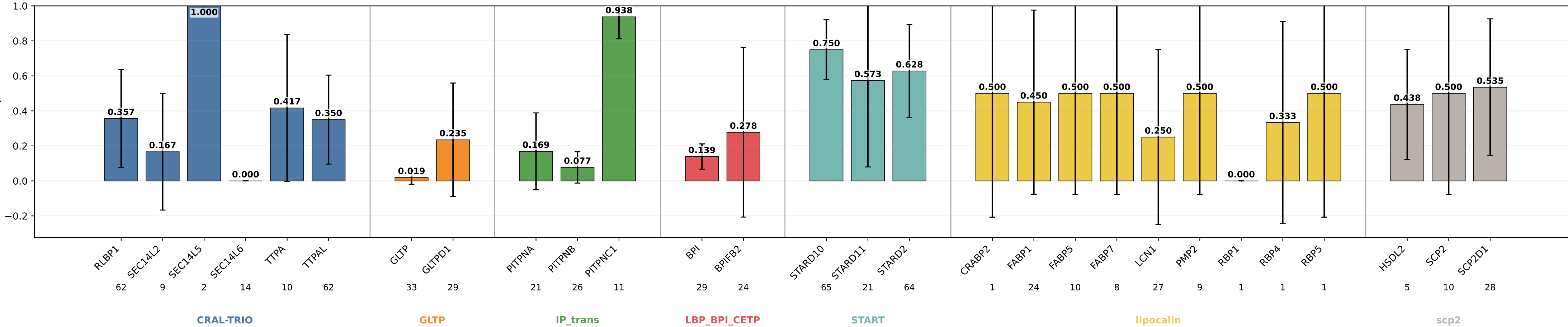
bbp_dcs_rand_smd_fa_nps_bilinear_fusion_dpt01_gm_plm8_hid8_wd001_lre-5_ep120 sensitivity by subgroup bbp_dcs_rand_smd_fa_nps_bilinear_fusion_dpt01_gm_plm8_hid8_wd001_lre-5_ep120 | class weights | lr=1e-05 | weight_decay=0.01 | final_m=4 | final_dropout=0.1 | hiddim=8 | heads=8 | batch=16 | ep=120 | seeds=0,1,2,3
