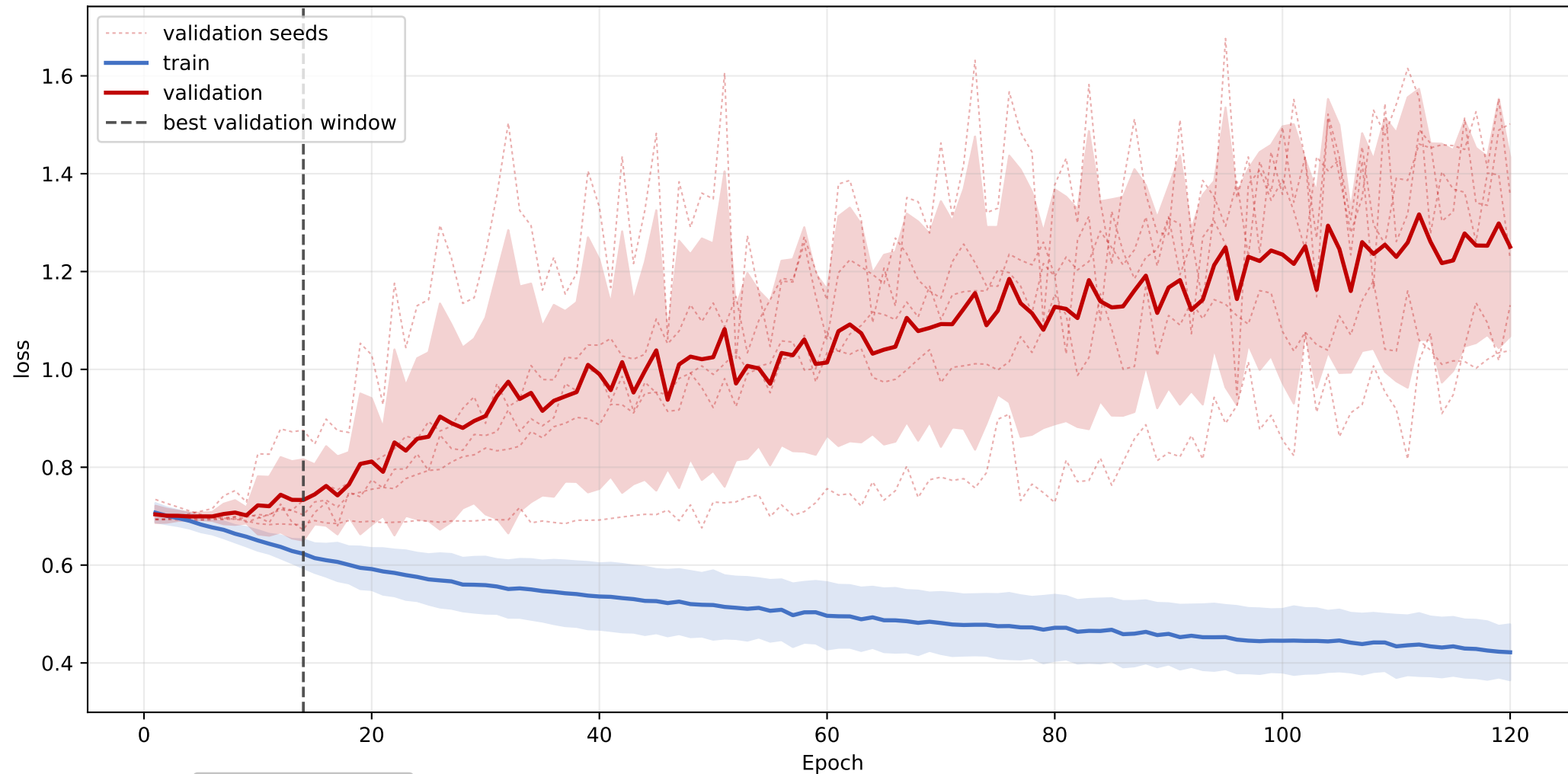
GLTP: mean loss learning curve across seeds
