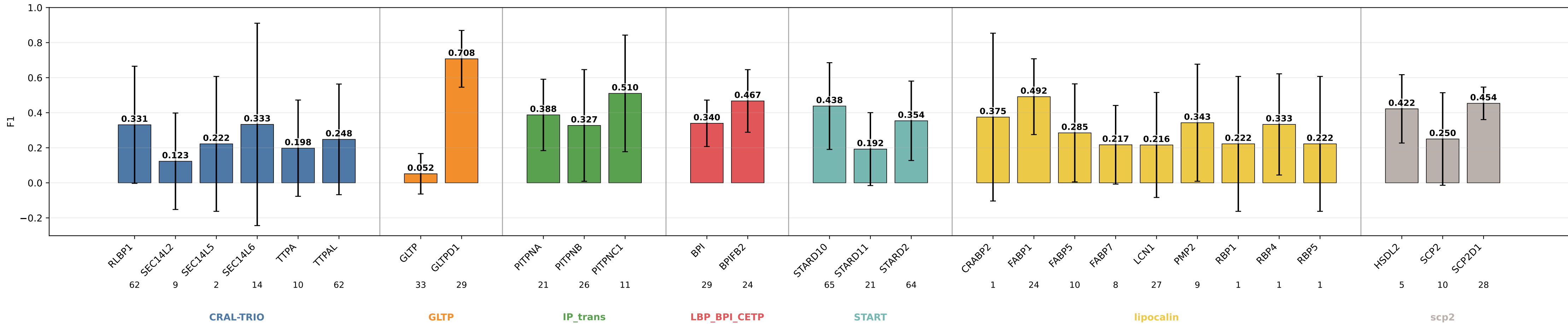
bbp_dcs_rand_smd_fa_nps_dpt01_gm_plm8_hid8_wd001_ep120 F1 by subgroup bbp_dcs_rand_smd_fa_nps_dpt01_gm_plm8_hid8_wd001_ep120 | class weights | lr=0.0001 | weight_decay=0.01 | final_m=4 | final_dropout=0.1 | hiddim=8 | heads=8 | batch=16 | ep=120 | seeds=0,1,2,3,4
