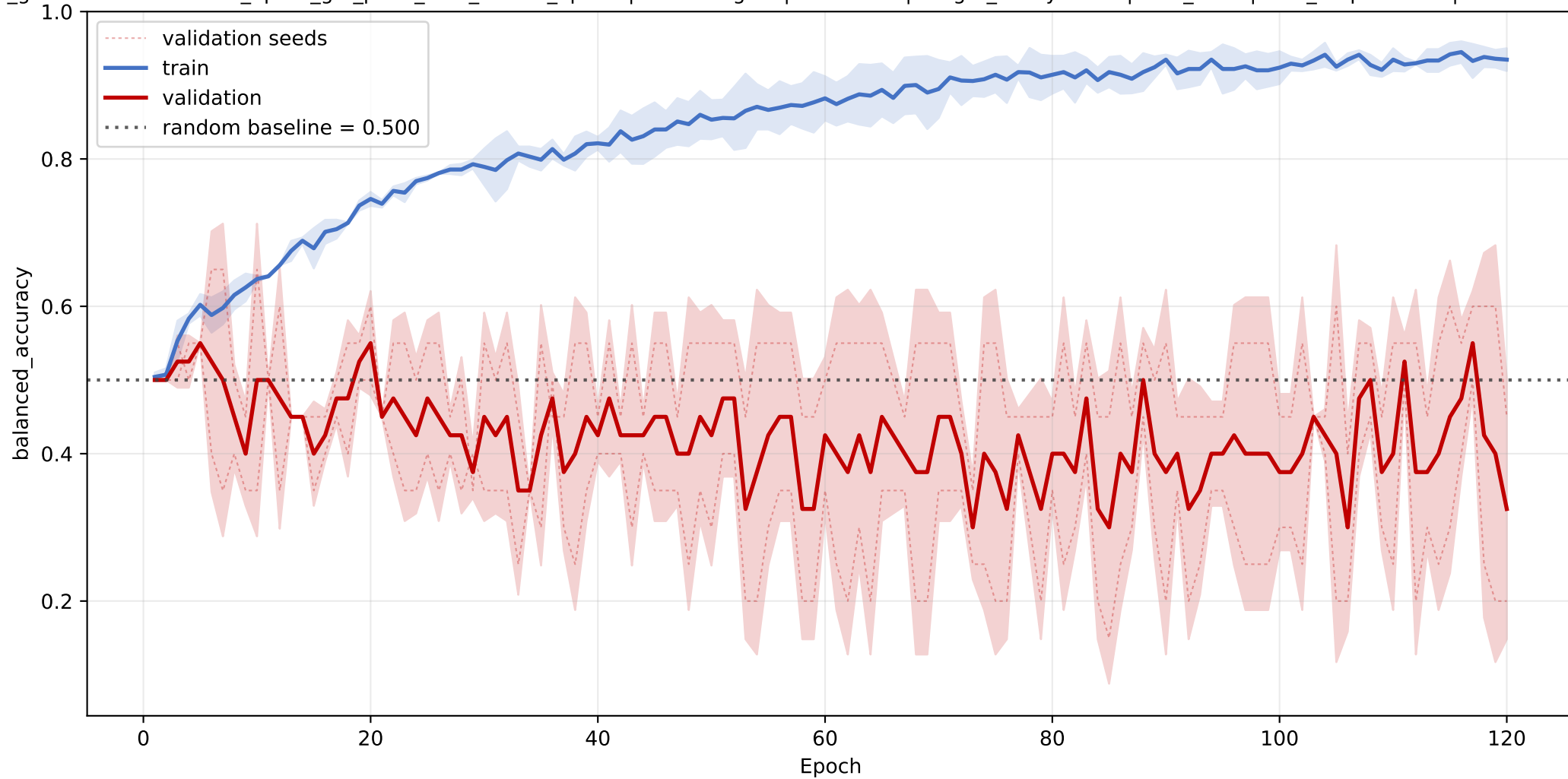
ML: mean balanced_accuracy learning curve across seeds
