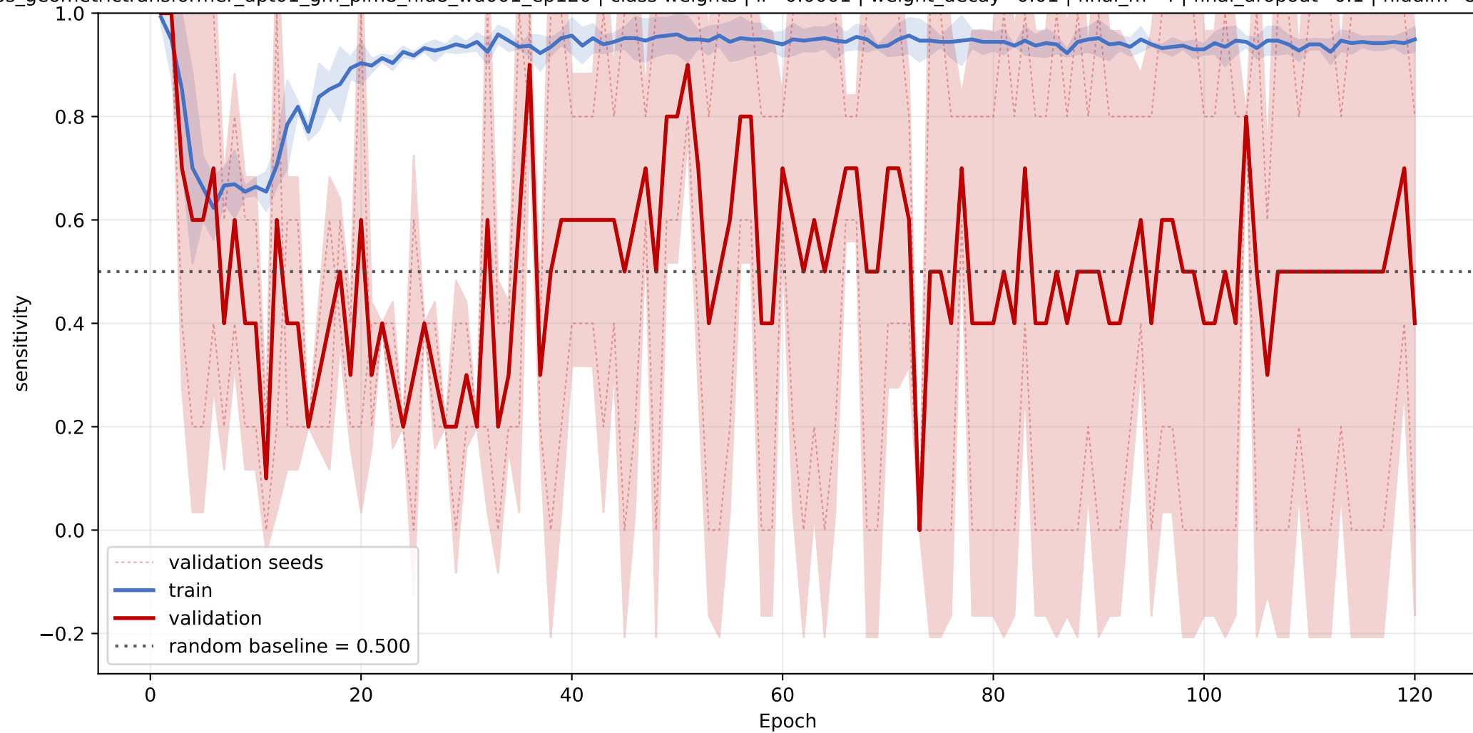
ML: mean sensitivity learning curve across seeds
