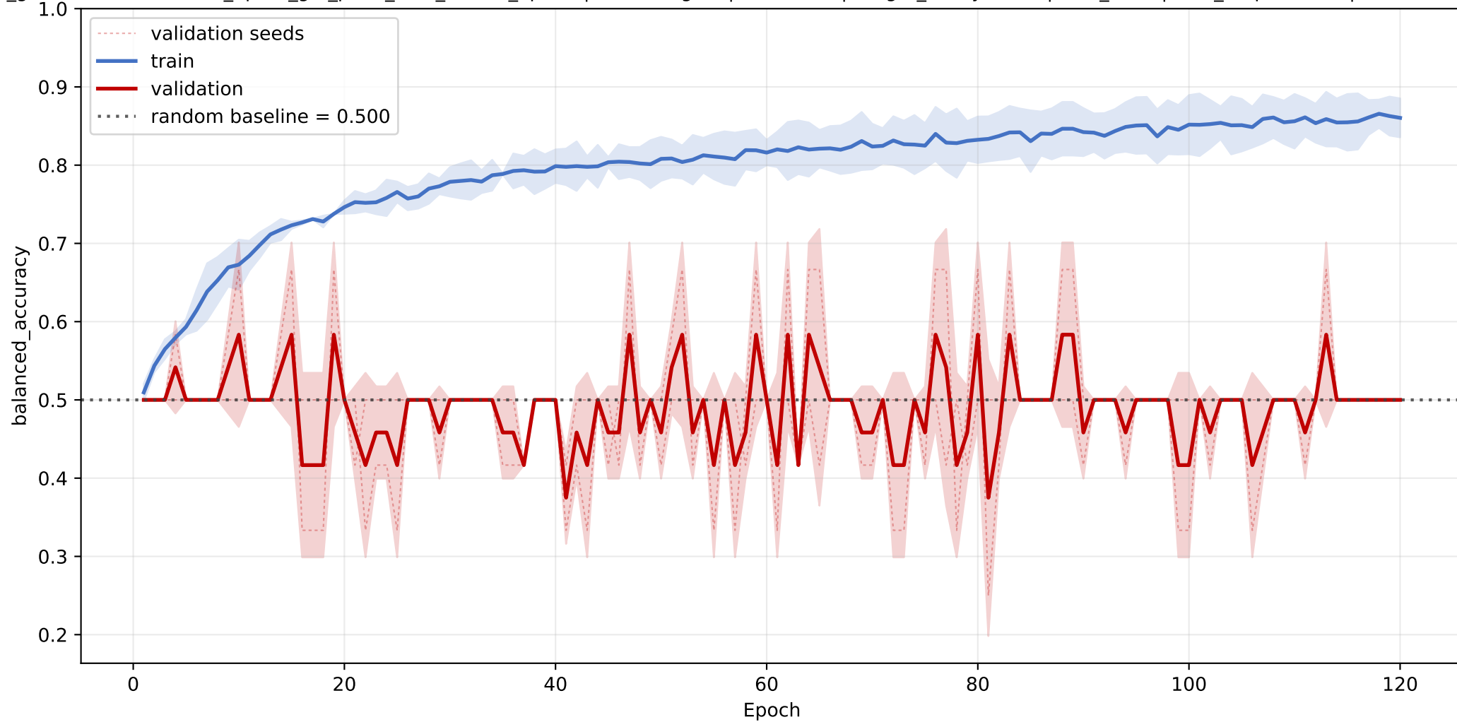
OSBP: mean balanced_accuracy learning curve across seeds
