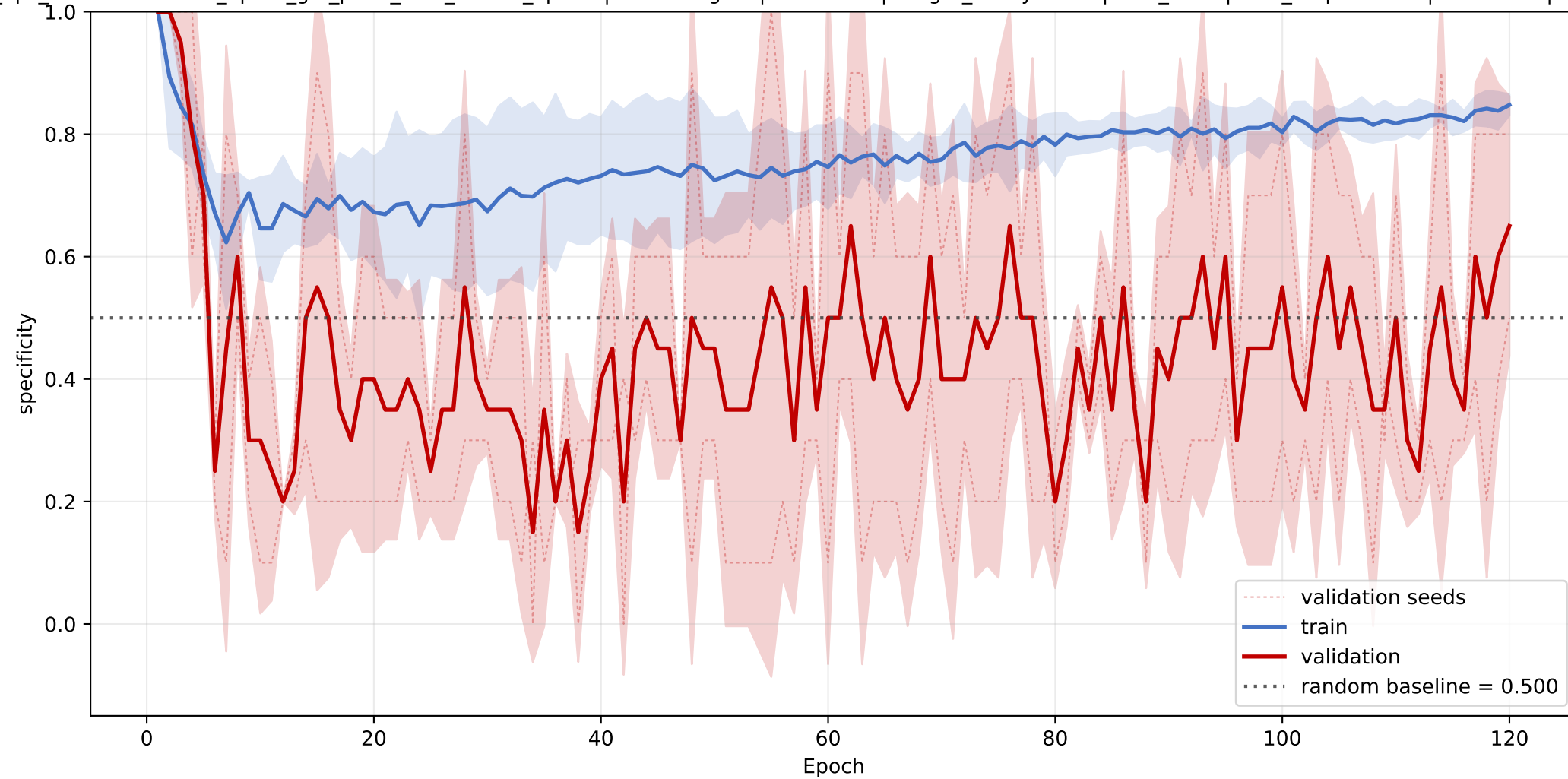
ML: mean specificity learning curve across seeds
