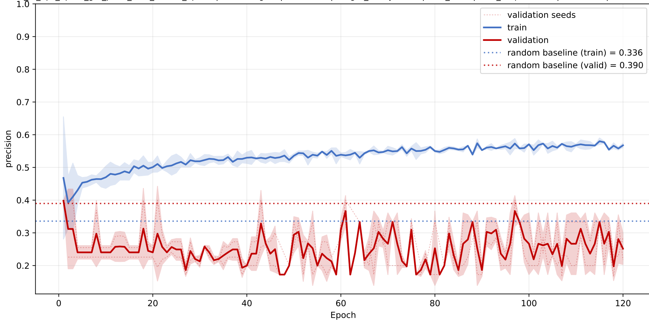
lipocalin: mean precision learning curve across seeds
