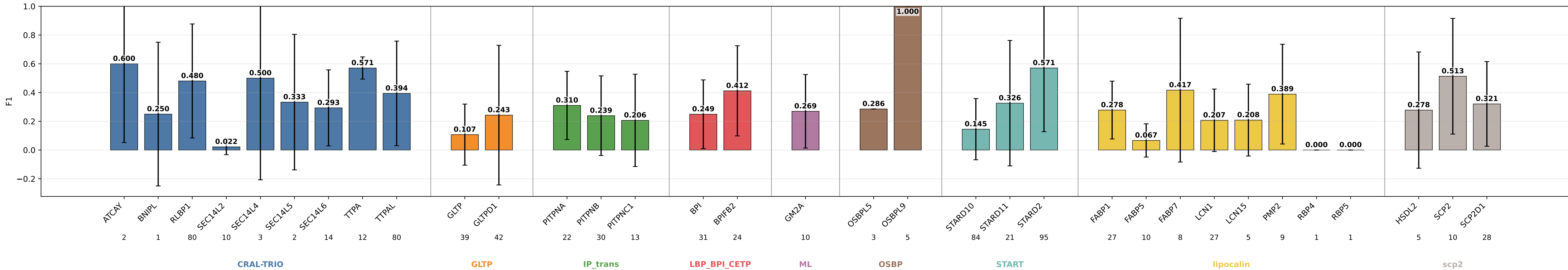
bbp_dcs_smd_fa_nps_clashonly_dpt01_gm_plm8_hid8_wd001_ep120 F1 by subgroup bbp_dcs_smd_fa_nps_clashonly_dpt01_gm_plm8_hid8_wd001_ep120 | class weights | lr=0.0001 | weight_decay=0.01 | final_m=4 | final_dropout=0.1 | hiddim=8 | heads=8 | batch=16 | ep=120 | seeds=0,1
