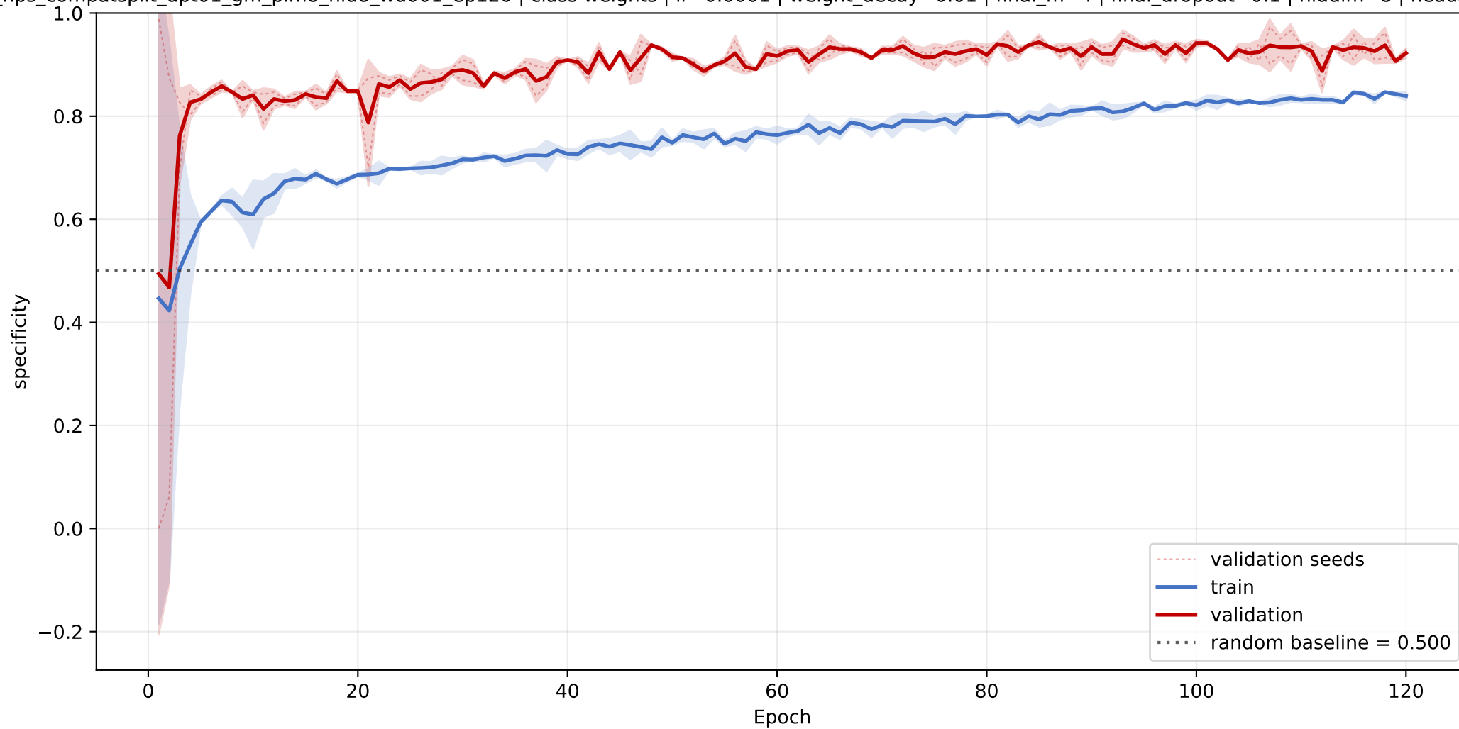
lipocalin: mean specificity learning curve across seeds
