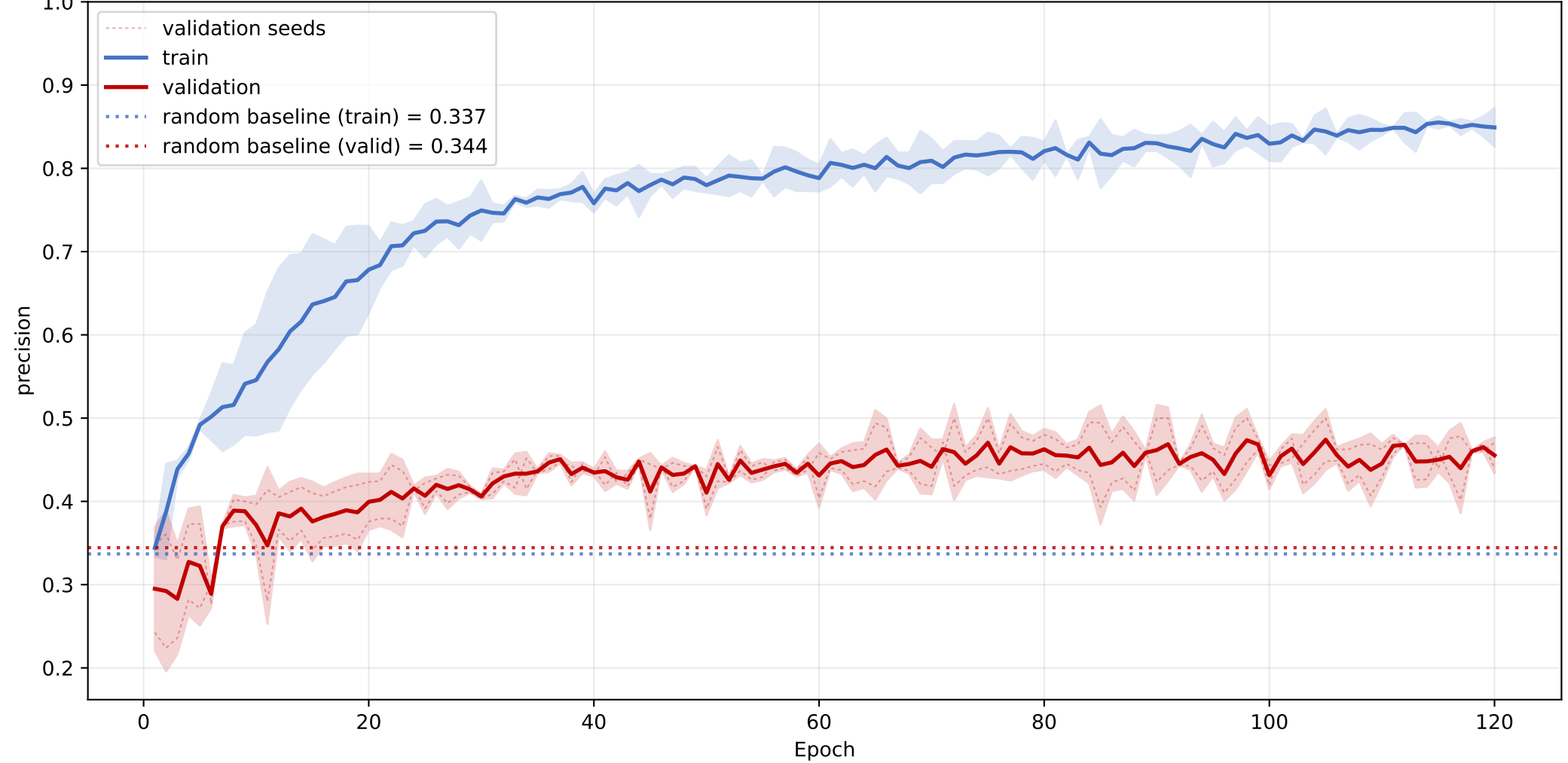
scp2: mean precision learning curve across seeds
