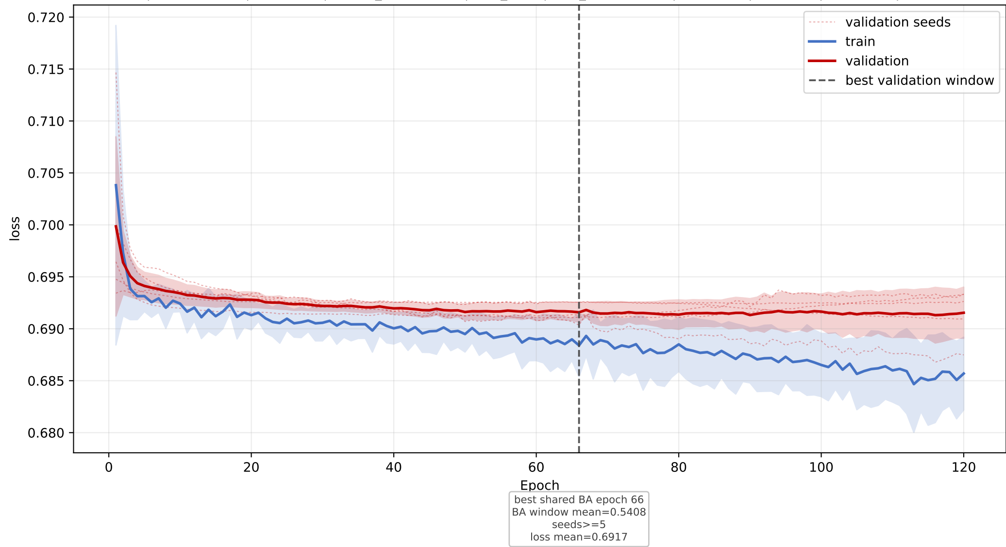
GLTP: mean loss learning curve across seeds
