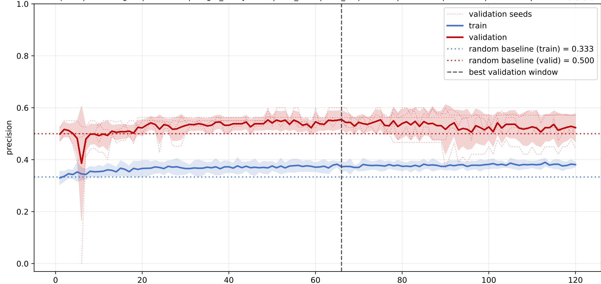
GLTP: mean precision learning curve across seeds
