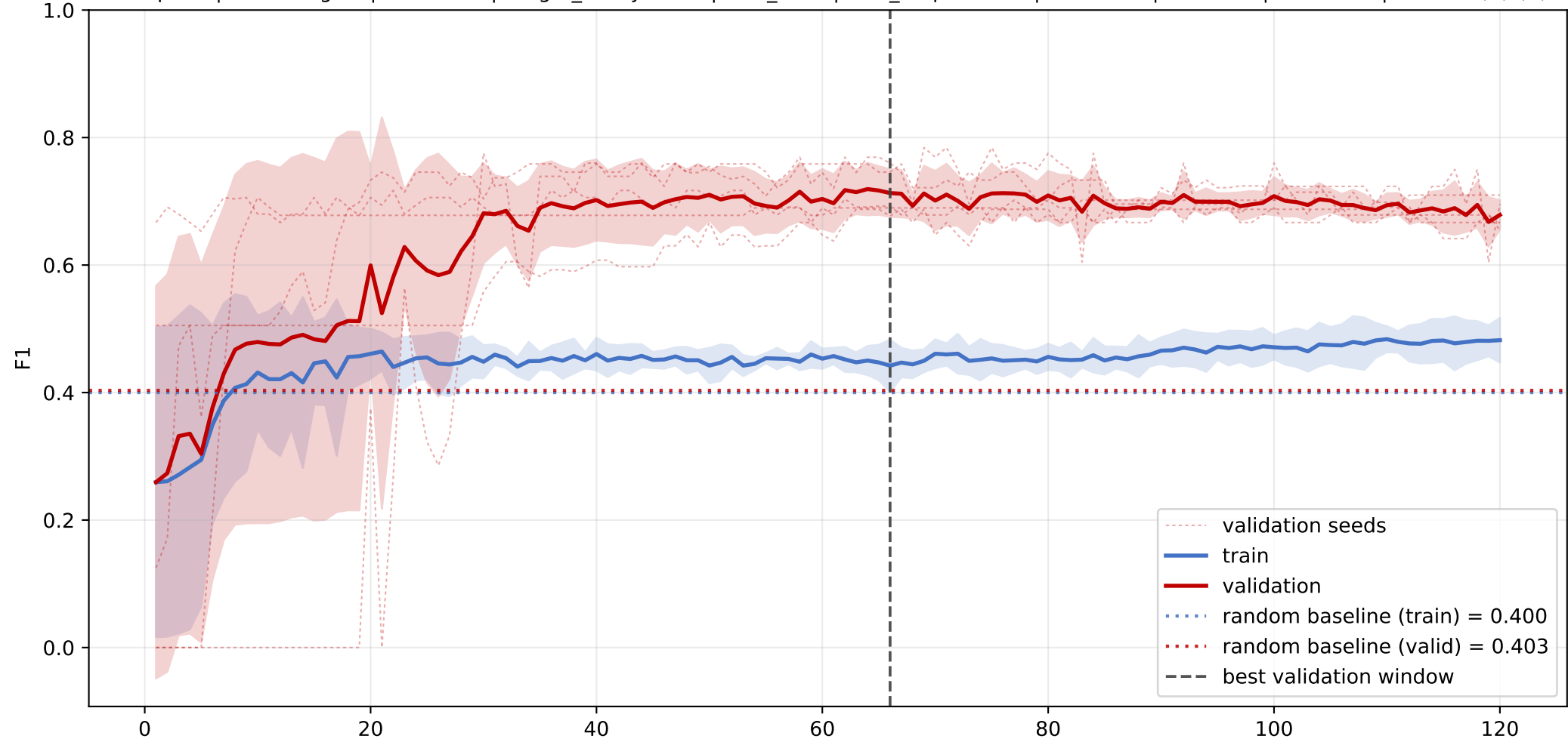
LBP_BPI_CETP: mean F1 learning curve across seeds
