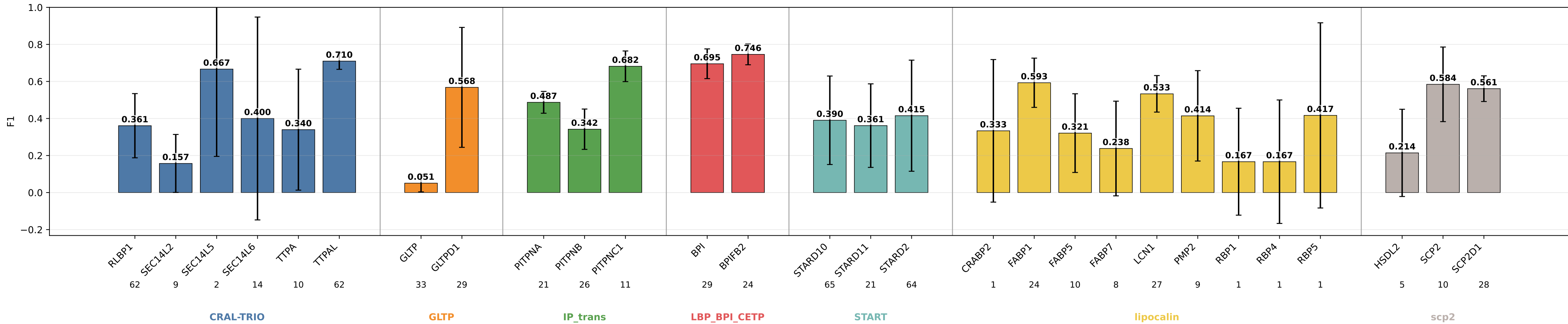
descriptors F1 by subgroup descriptors | class weights | lr=0.0001 | weight_decay=0.01 | final_m=4 | final_dropout=0.1 | hiddim=8 | heads=8 | batch=16 | ep=120 | seeds=0,1,2,3,4
