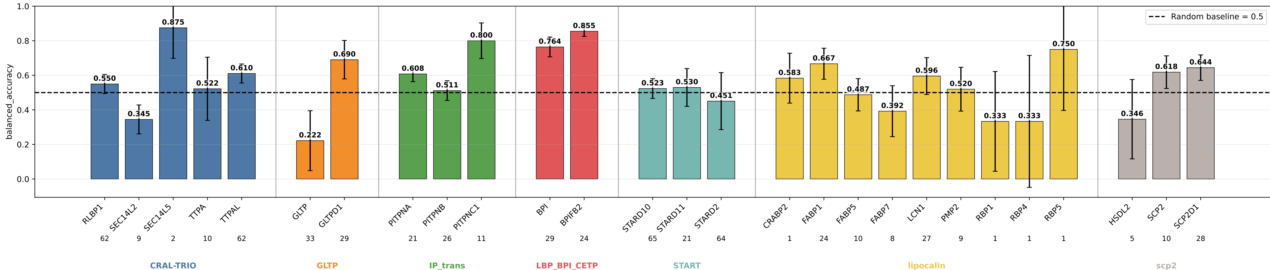
descriptors balanced_accuracy by subgroup descriptors | class weights | lr=0.0001 | weight_decay=0.01 | final_m=4 | final_dropout=0.1 | hiddim=8 | heads=8 | batch=16 | ep=120 | seeds=0,1,2,3,4
