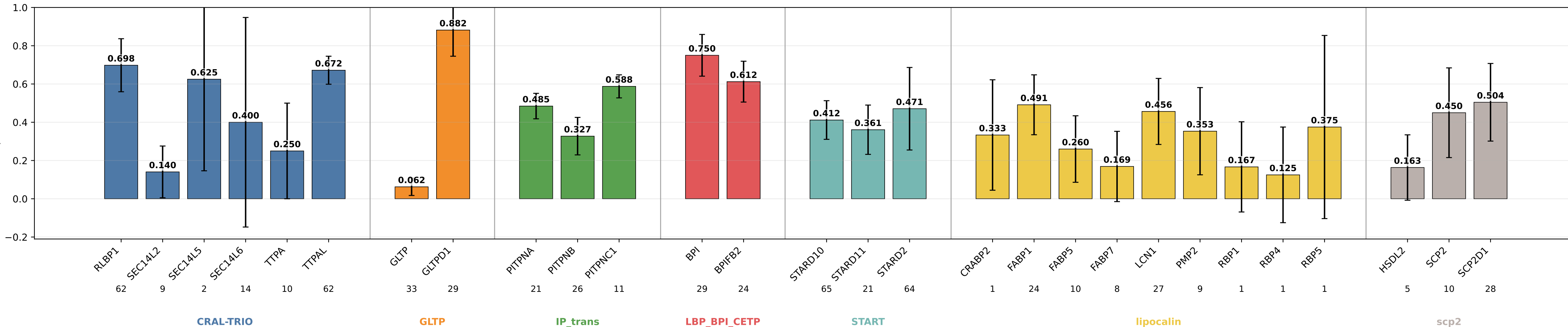
descriptors precision by subgroup descriptors | class weights | lr=0.0001 | weight_decay=0.01 | final_m=4 | final_dropout=0.1 | hiddim=8 | heads=8 | batch=16 | ep=120 | seeds=0,1,2,3,4
