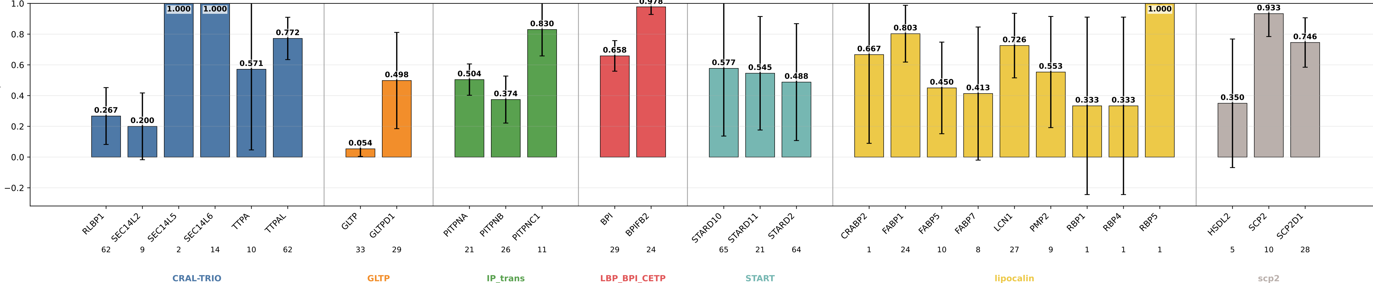
descriptors sensitivity by subgroup descriptors | class weights | lr=0.0001 | weight_decay=0.01 | final_m=4 | final_dropout=0.1 | hiddim=8 | heads=8 | batch=16 | ep=120 | seeds=0,1,2,3,4
