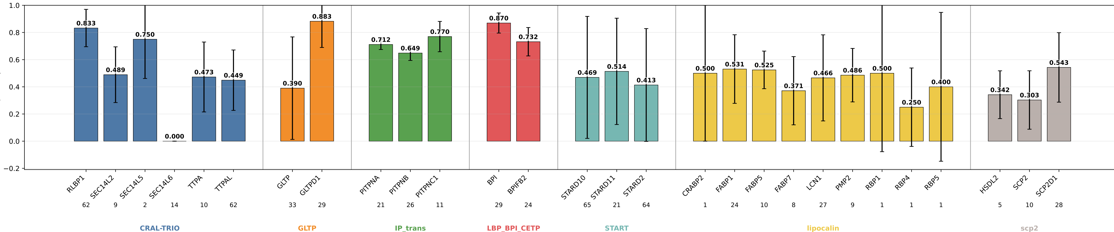
descriptors specificity by subgroup descriptors | class weights | lr=0.0001 | weight_decay=0.01 | final_m=4 | final_dropout=0.1 | hiddim=8 | heads=8 | batch=16 | ep=120 | seeds=0,1,2,3,4
