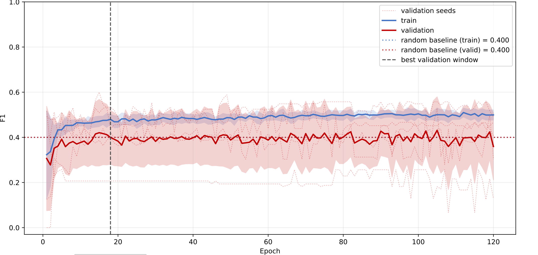
scp2: mean F1 learning curve across seeds
