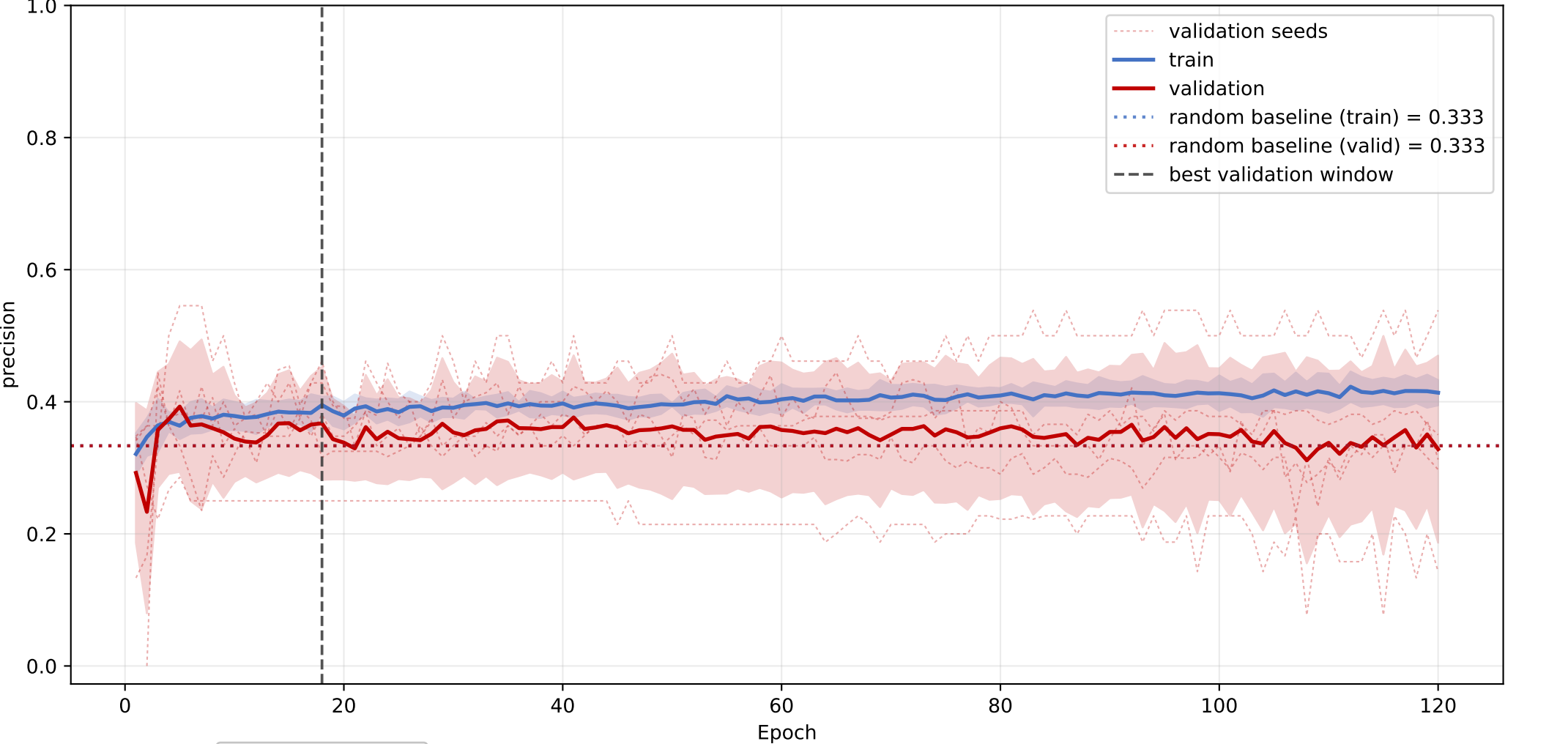
scp2: mean precision learning curve across seeds
